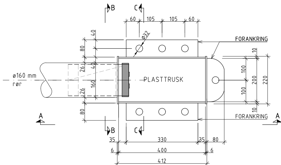
PLAN PLASTTRUSK
