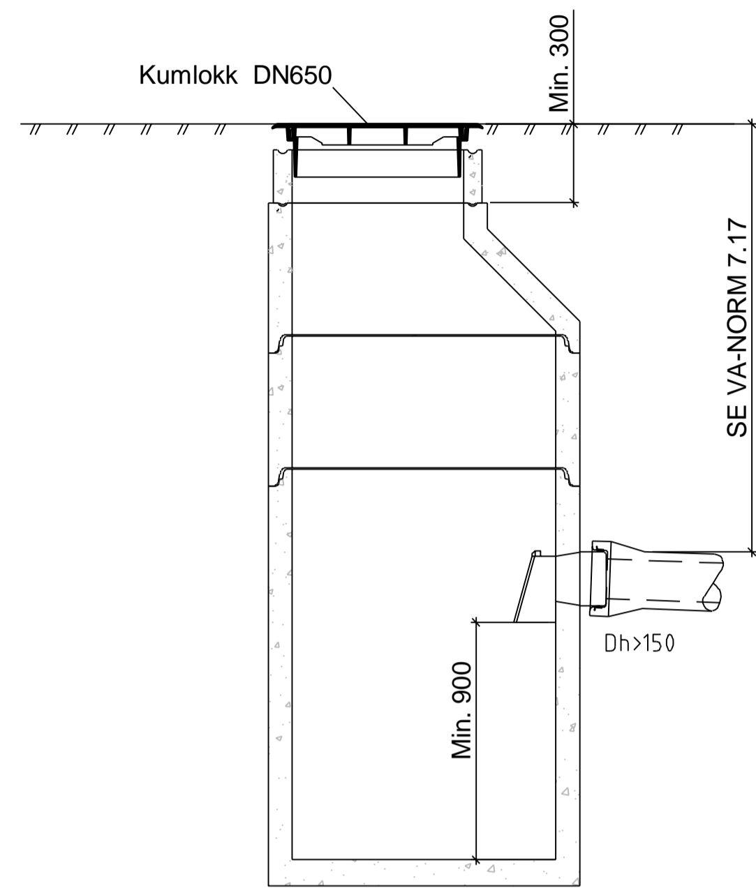
SNITT SANDFANGKUM BETONG 1000 MM - 120 -
