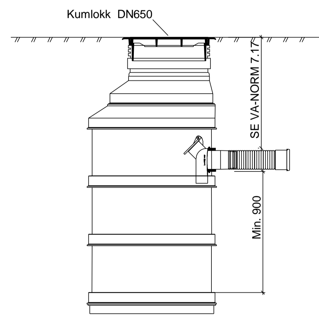
SNITT SANDFANGKUM PLAST 1000 MM - 120 -
