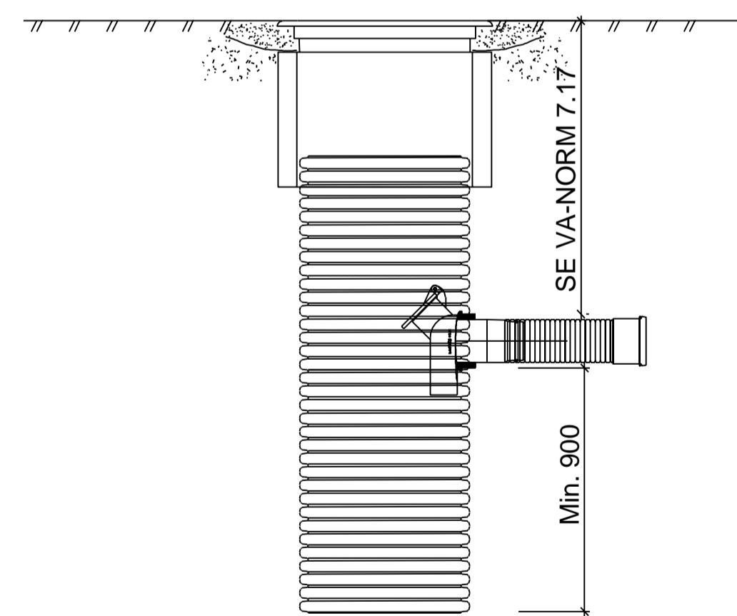
SNITT SANDFANGKUM PLAST 600/630 MM - 120 -
