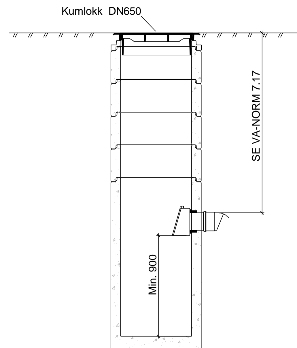
SNITT SANDFANGKUM BETONG 650 MM - 120 -
